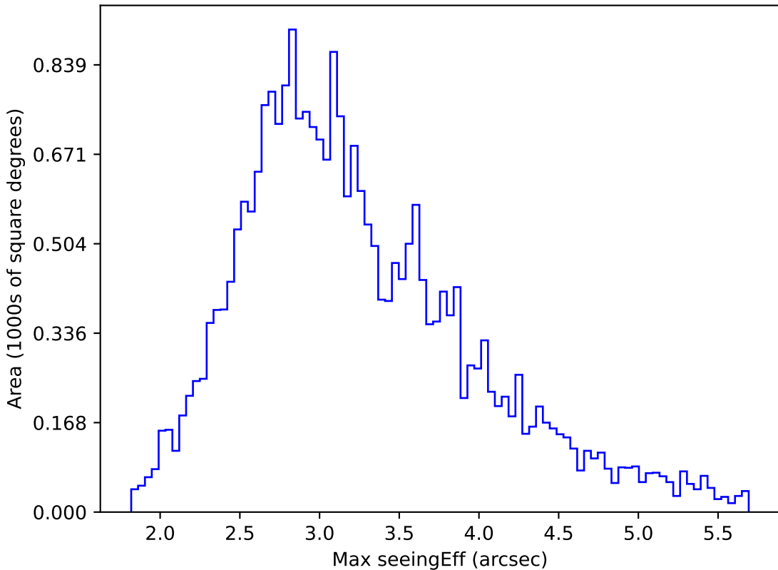
roll_pause_mjdp120_v3.4_10yrs All sky all bands: Max seeingEff
