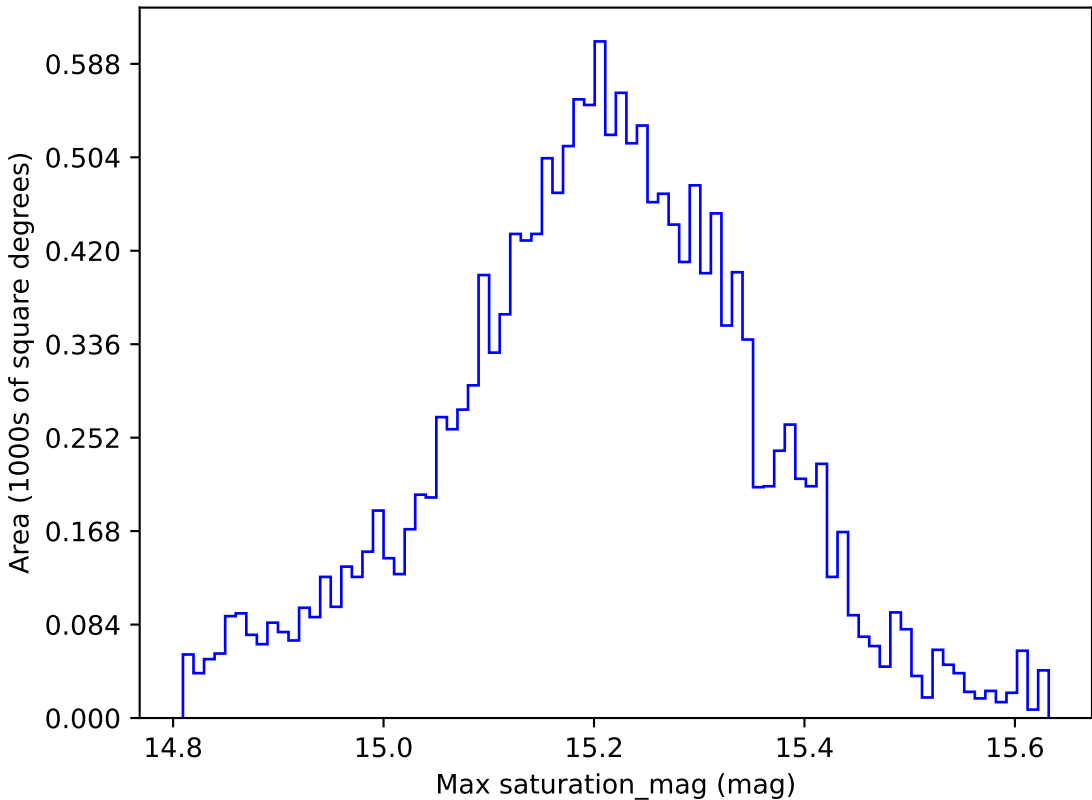
roll_pause_mjdp120_v3.4_10yrs WFD z band: Max saturation_mag
