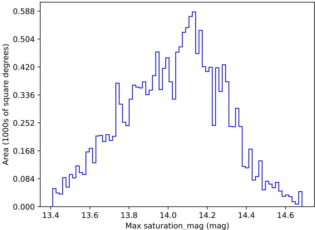
roll_pause_mjdp120_v3.4_10yrs WFD u band: Max saturation_mag
