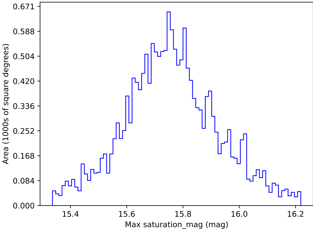
roll_pause_mjdp120_v3.4_10yrs WFD r band: Max saturation_mag
