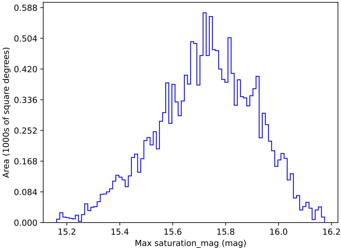
roll_pause_mjdp120_v3.4_10yrs WFD g band: Max saturation_mag
