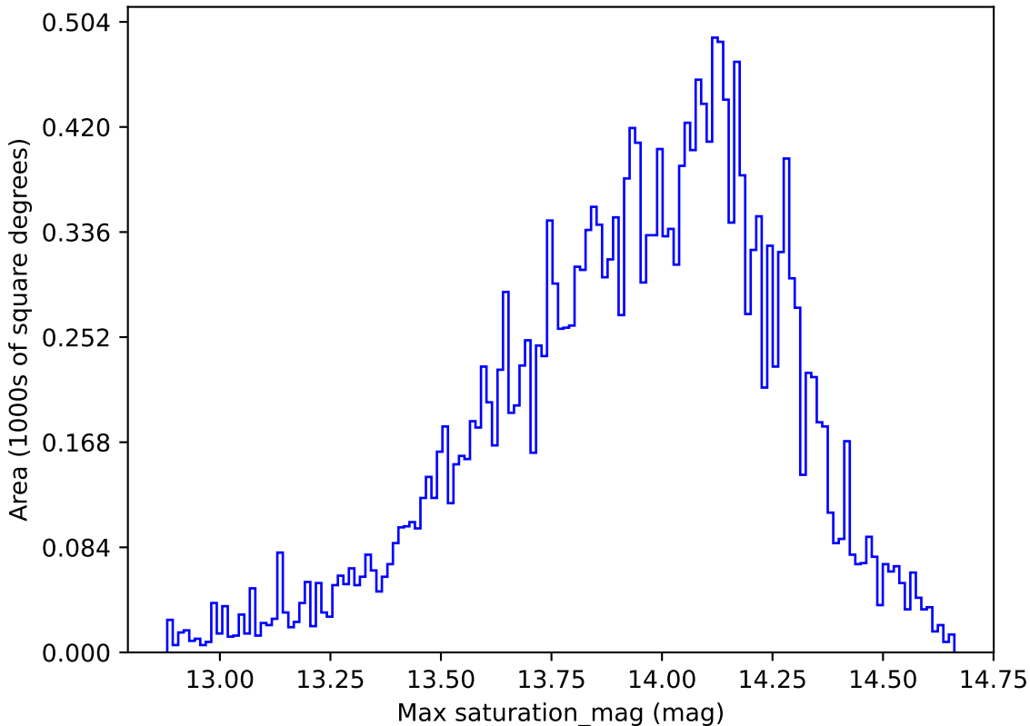
roll_pause_mjdp120_v3.4_10yrs All sky u band: Max saturation_mag
