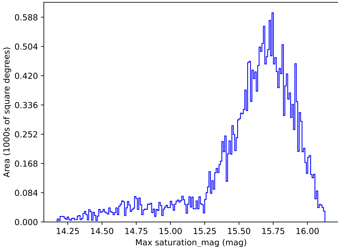
roll_pause_mjdp120_v3.4_10yrs All sky g band: Max saturation_mag
