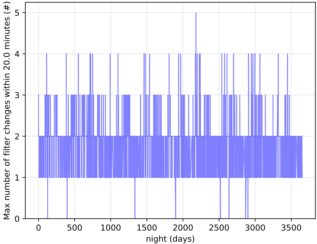
roll_pause_mjdp120_v3.4_10yrs Per Night: Max number of filter changes within 20.0 minutes
