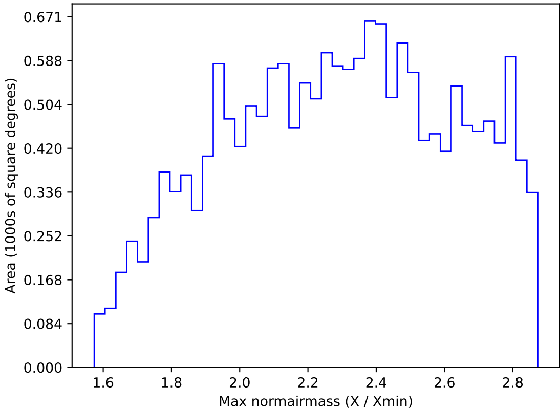
roll_pause_mjdp120_v3.4_10yrs WFD z band: Max normairmass
