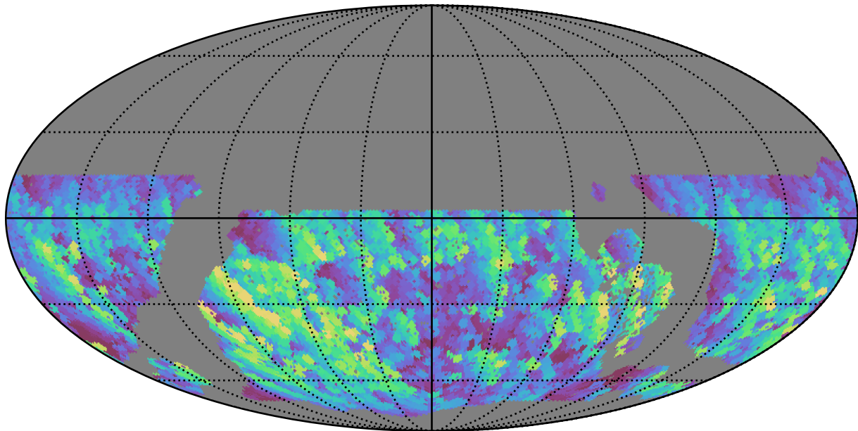
roll_pause_mjdp120_v3.4_10yrs WFD y band: Max normairmass
