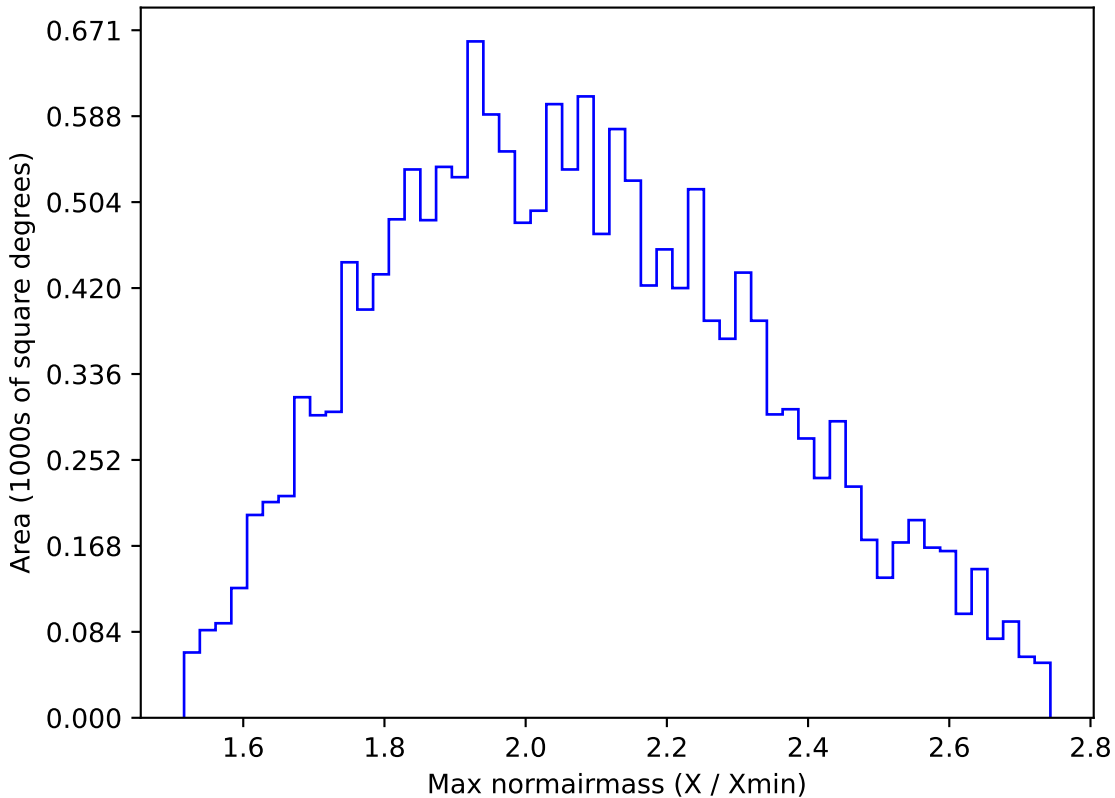
roll_pause_mjdp120_v3.4_10yrs WFD y band: Max normairmass
