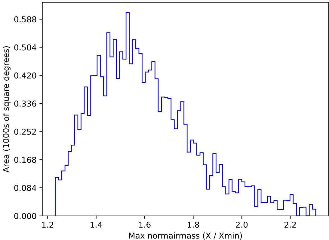
roll_pause_mjdp120_v3.4_10yrs WFD u band: Max normairmass
