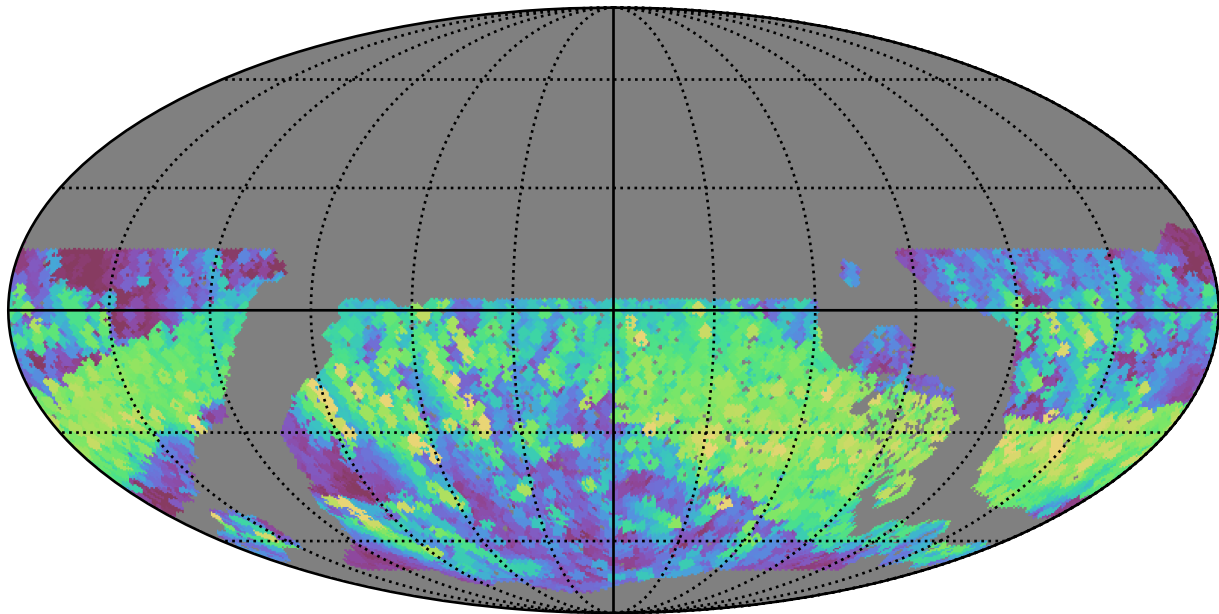
roll_pause_mjdp120_v3.4_10yrs WFD r band: Max normairmass
