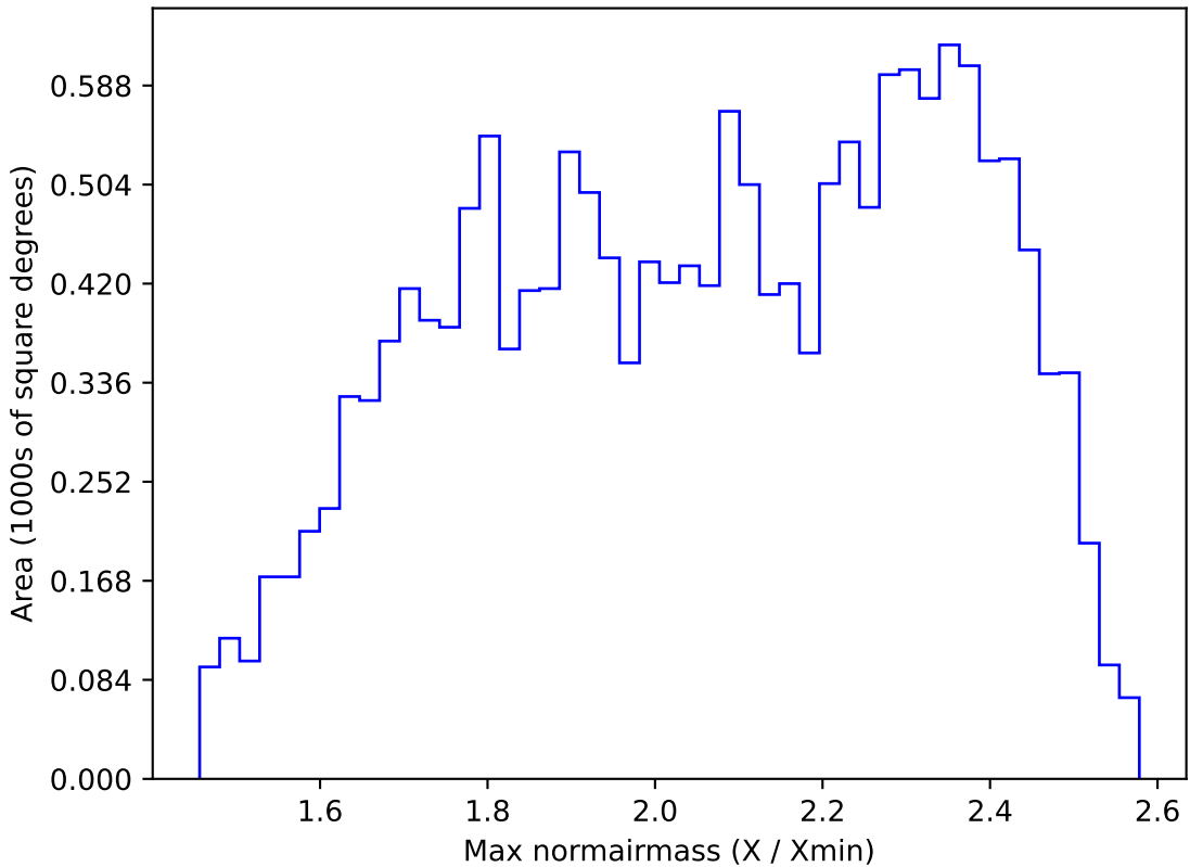
roll_pause_mjdp120_v3.4_10yrs WFD r band: Max normairmass
