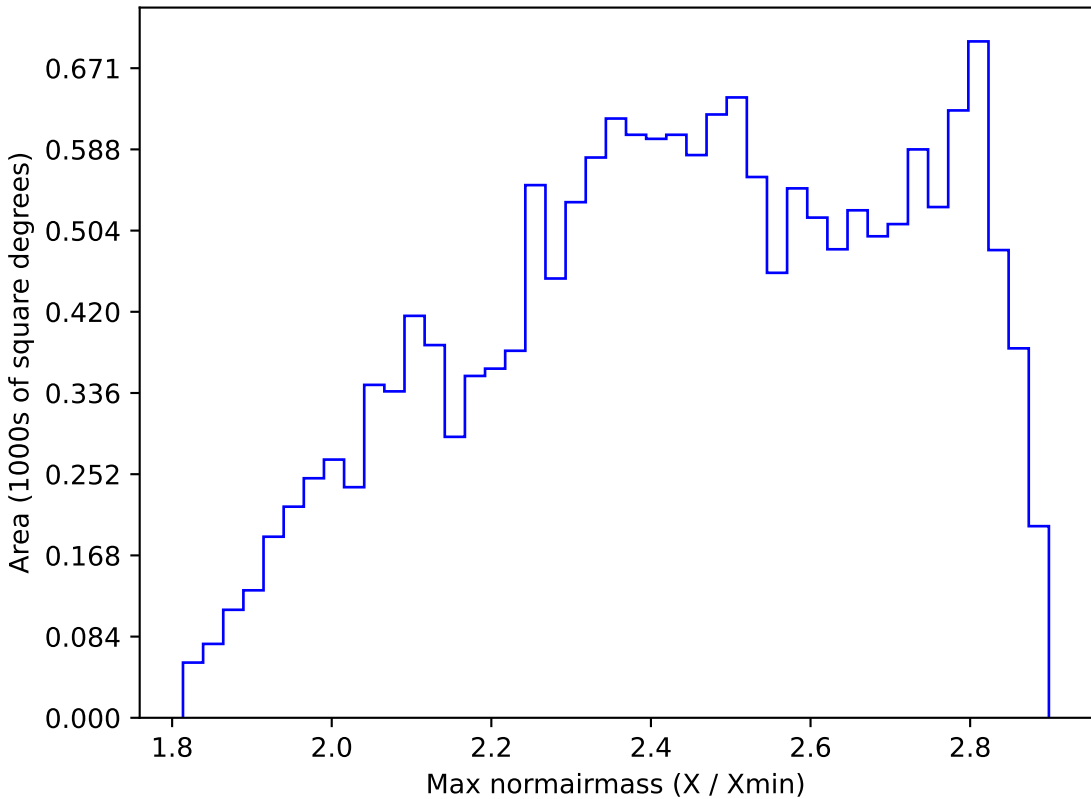
roll_pause_mjdp120_v3.4_10yrs WFD all bands: Max normairmass
