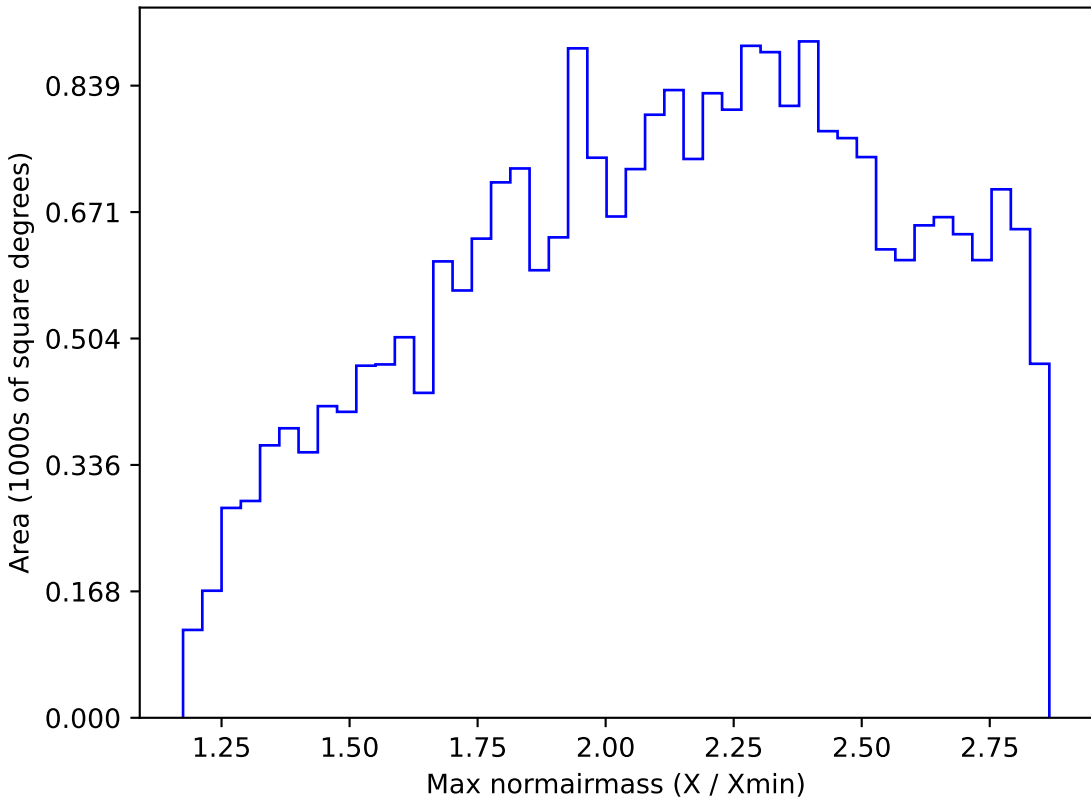
roll_pause_mjdp120_v3.4_10yrs All sky z band: Max normairmass
