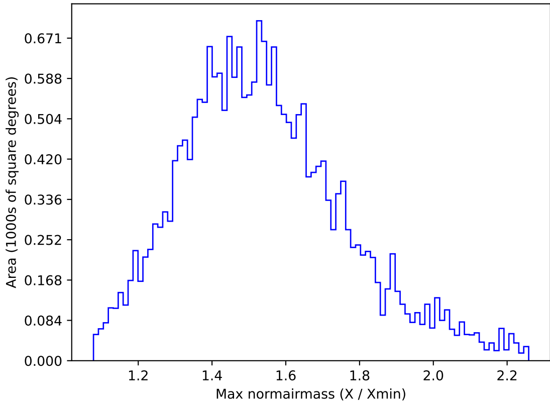
roll_pause_mjdp120_v3.4_10yrs All sky u band: Max normairmass
