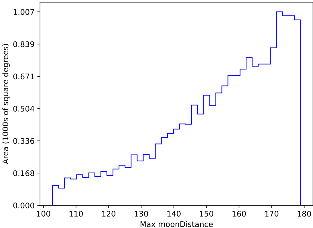
roll_pause_mjdp120_v3.4_10yrs WFD z band: Max moonDistance
