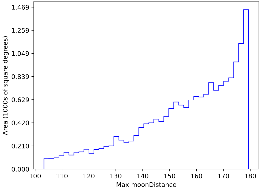
roll_pause_mjdp120_v3.4_10yrs WFD r band: Max moonDistance
