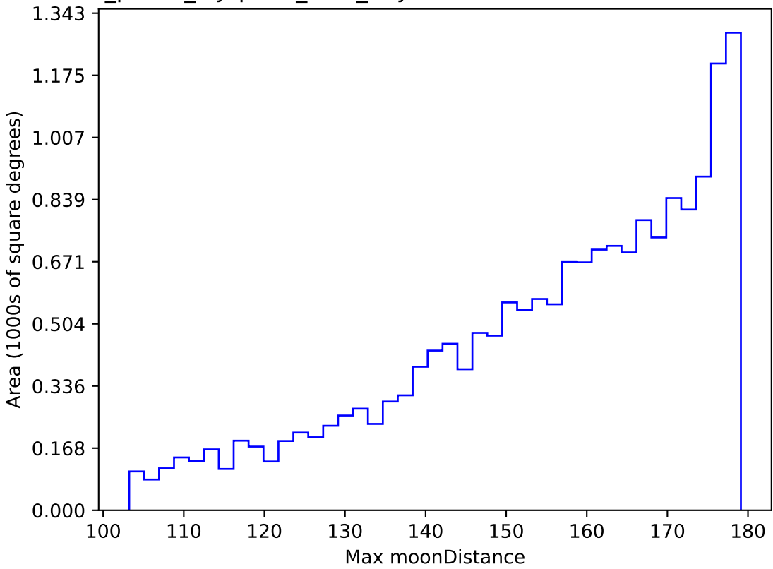
roll_pause_mjdp120_v3.4_10yrs WFD i band: Max moonDistance
