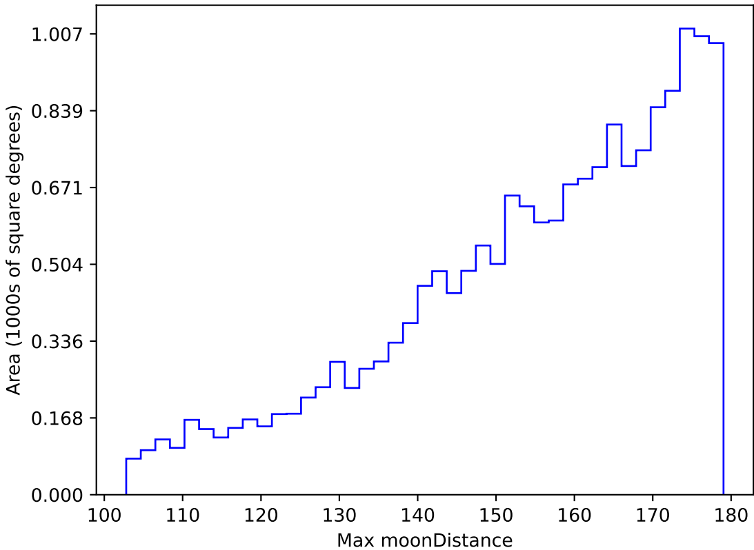
roll_pause_mjdp120_v3.4_10yrs WFD g band: Max moonDistance
