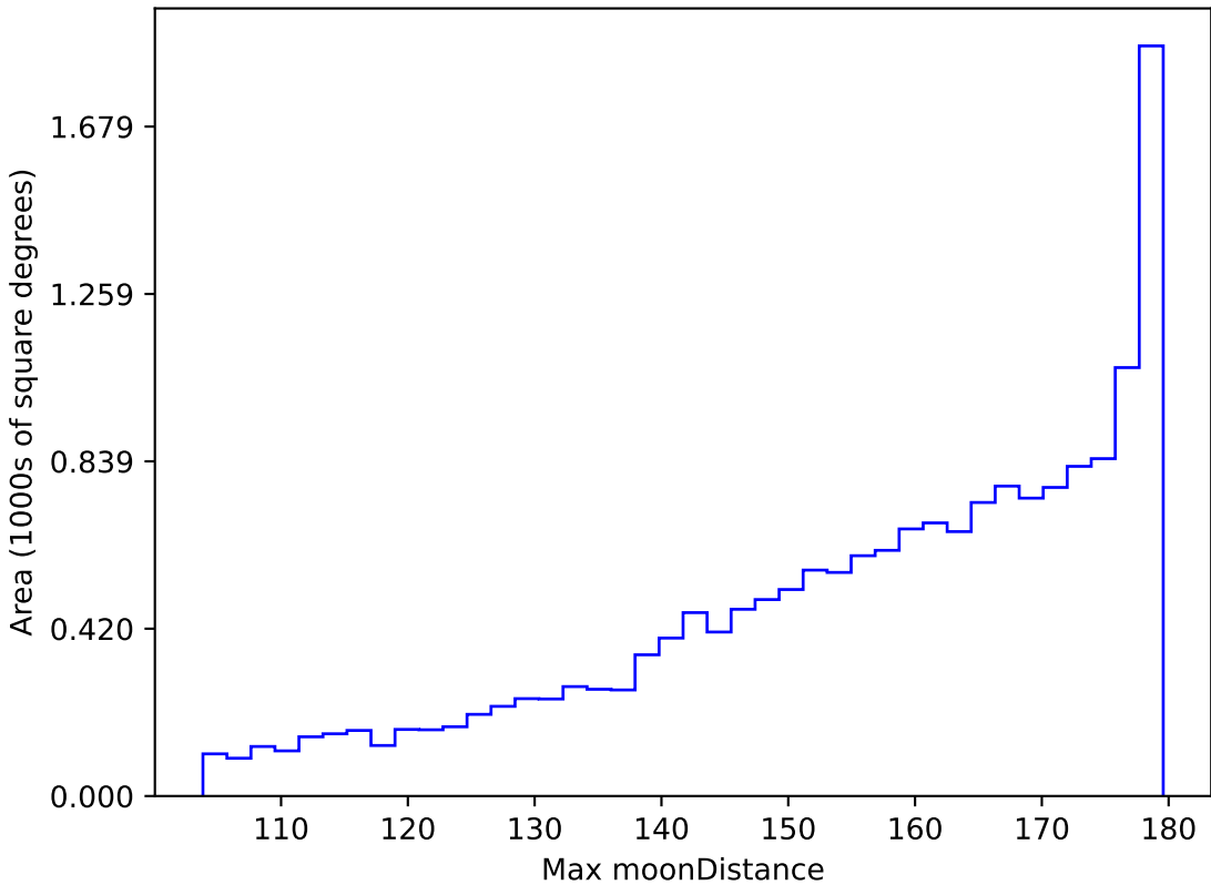
roll_pause_mjdp120_v3.4_10yrs WFD all bands: Max moonDistance
