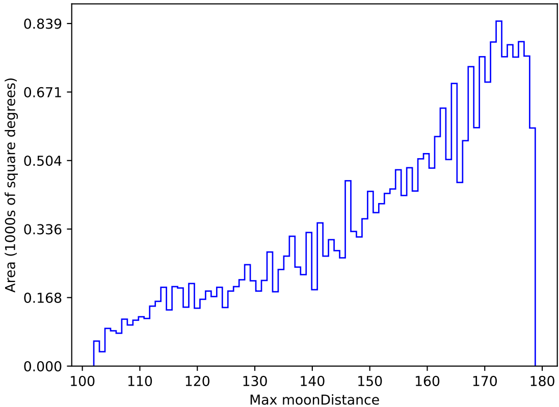
roll_pause_mjdp120_v3.4_10yrs All sky z band: Max moonDistance
