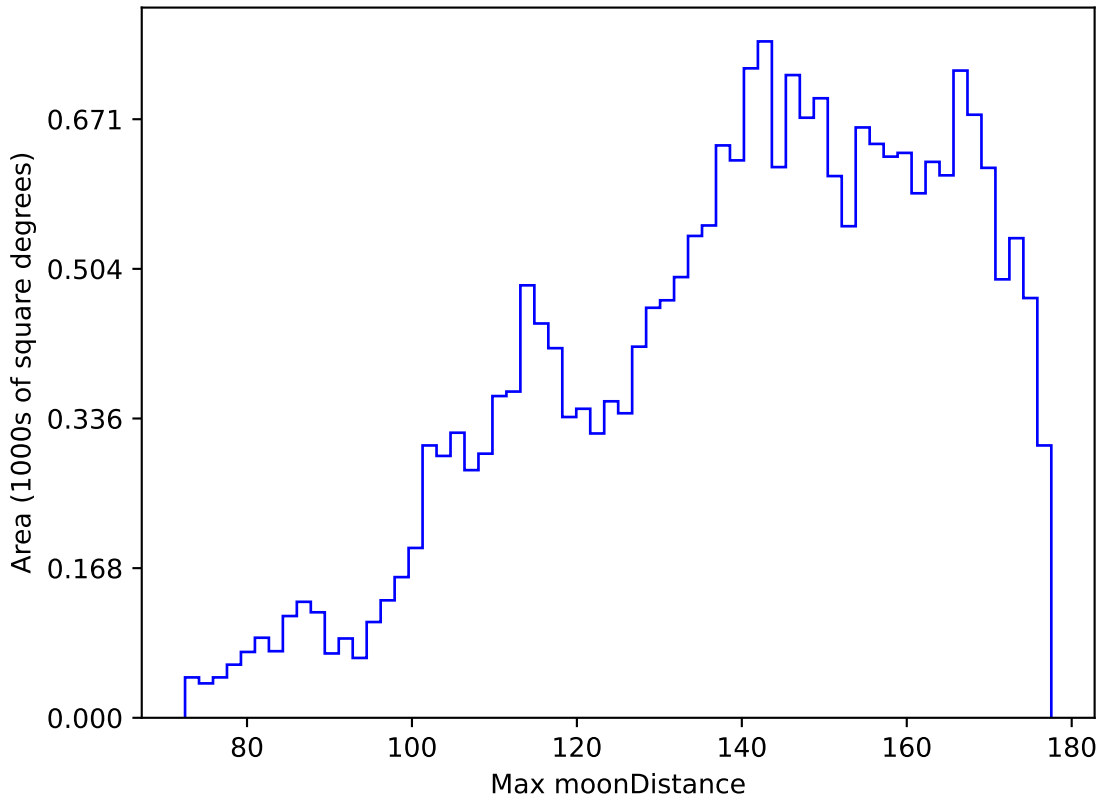
roll_pause_mjdp120_v3.4_10yrs All sky y band: Max moonDistance
