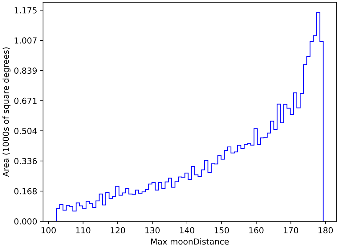
roll_pause_mjdp120_v3.4_10yrs All sky r band: Max moonDistance
