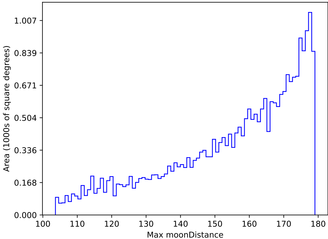
roll_pause_mjdp120_v3.4_10yrs All sky i band: Max moonDistance
