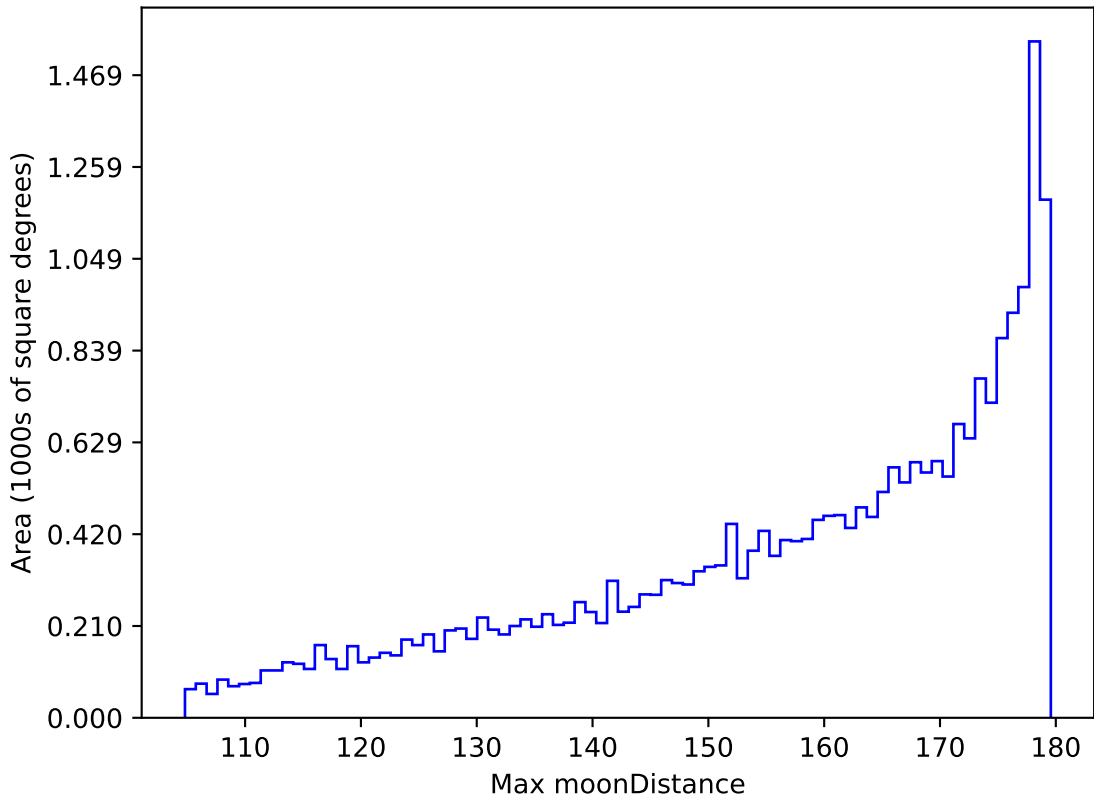
roll_pause_mjdp120_v3.4_10yrs All sky all bands: Max moonDistance
