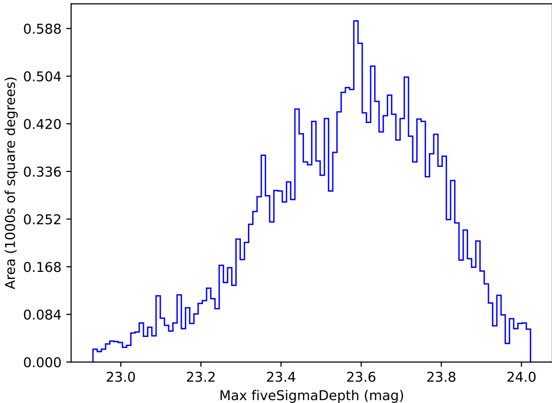
roll_pause_mjdp120_v3.4_10yrs Yr 1 u band: Max fiveSigmaDepth
