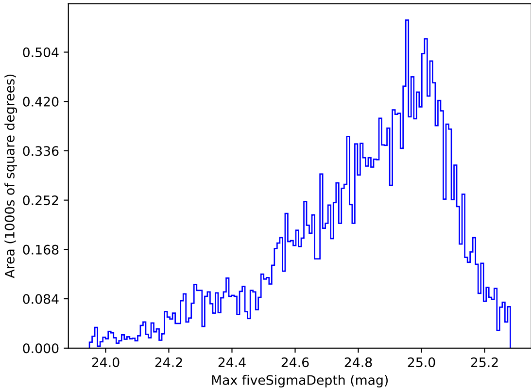
roll_pause_mjdp120_v3.4_10yrs Yr 1 g band: Max fiveSigmaDepth
