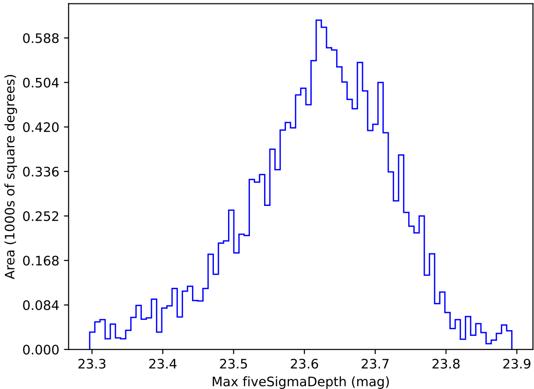
roll_pause_mjdp120_v3.4_10yrs WFD z band: Max fiveSigmaDepth
