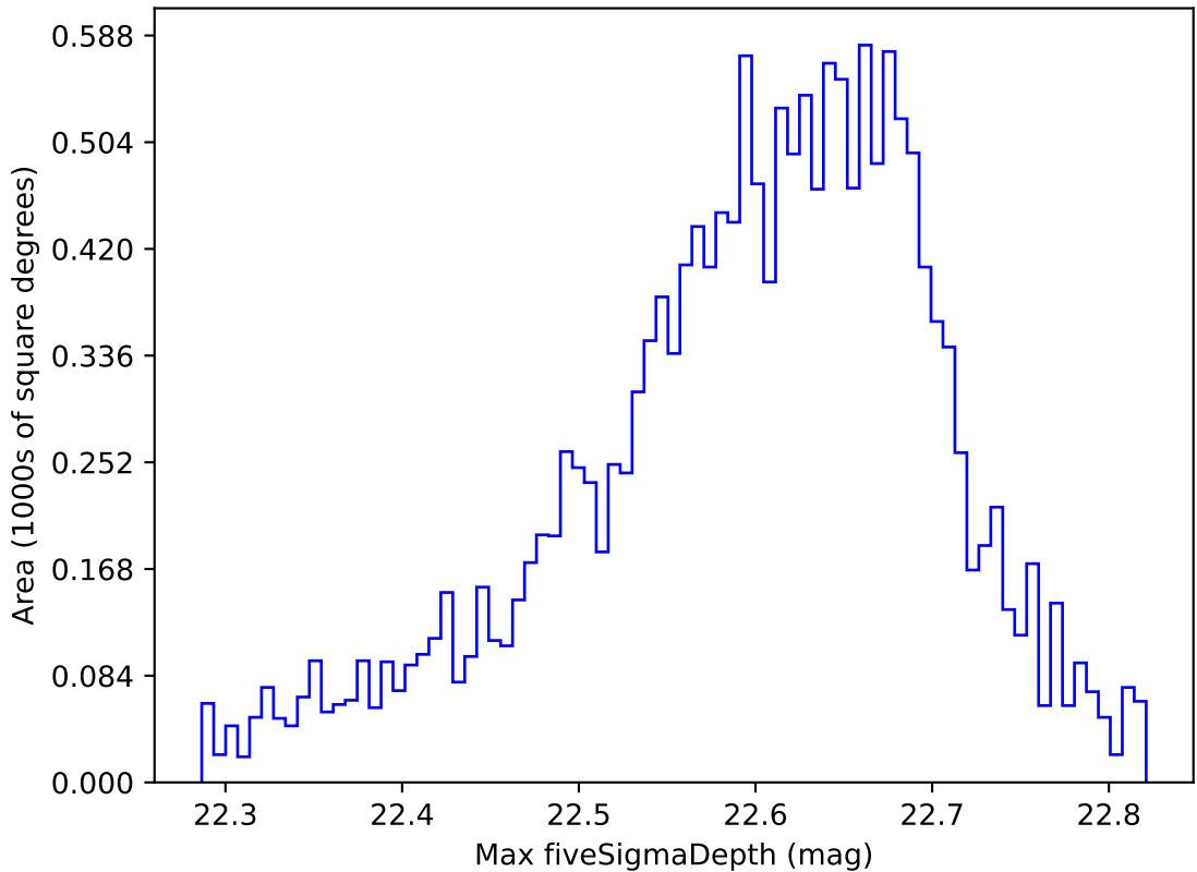
roll_pause_mjdp120_v3.4_10yrs WFD y band: Max fiveSigmaDepth
