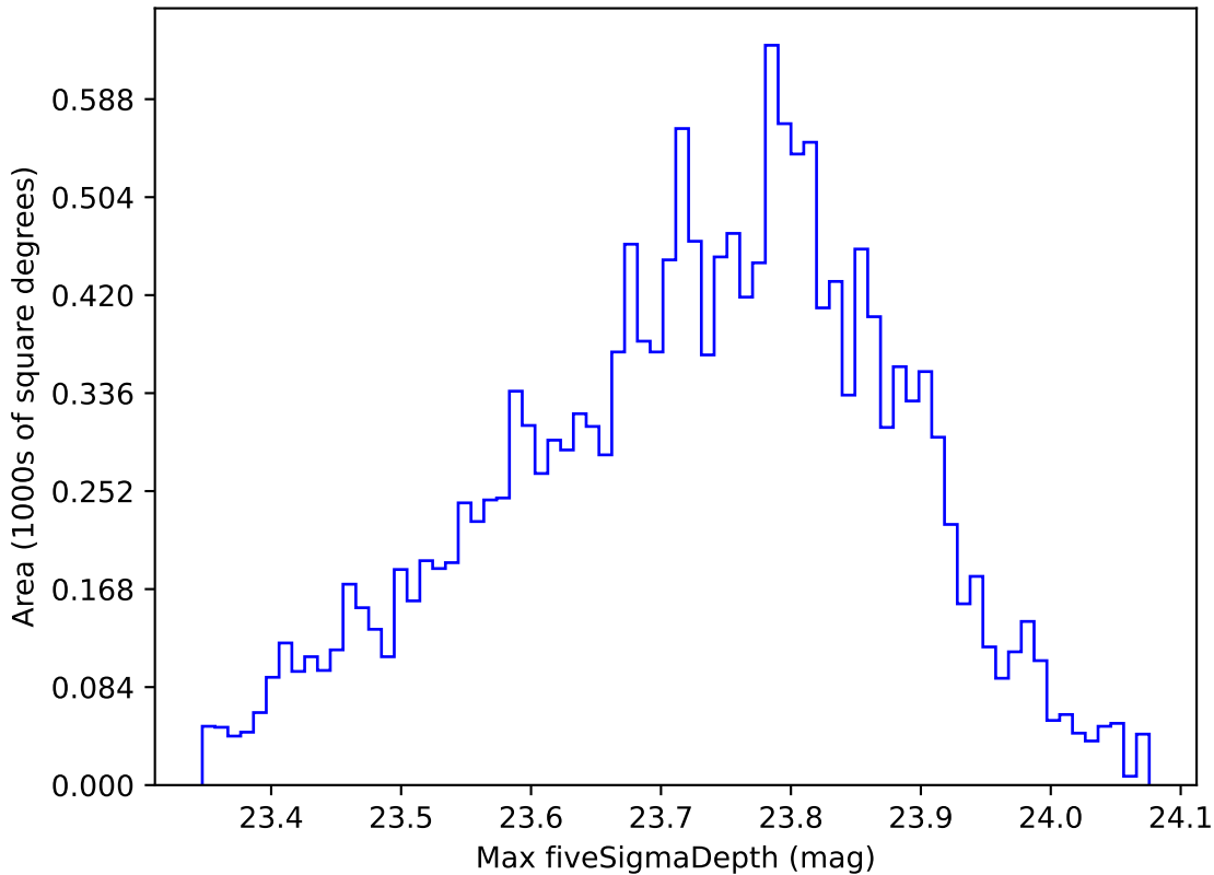
roll_pause_mjdp120_v3.4_10yrs WFD u band: Max fiveSigmaDepth
