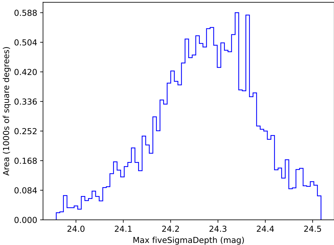
roll_pause_mjdp120_v3.4_10yrs WFD i band: Max fiveSigmaDepth
