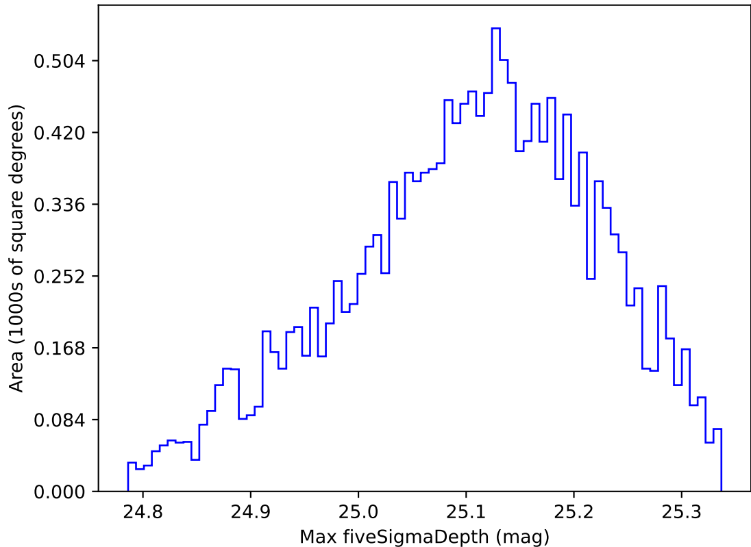
roll_pause_mjdp120_v3.4_10yrs WFD g band: Max fiveSigmaDepth
