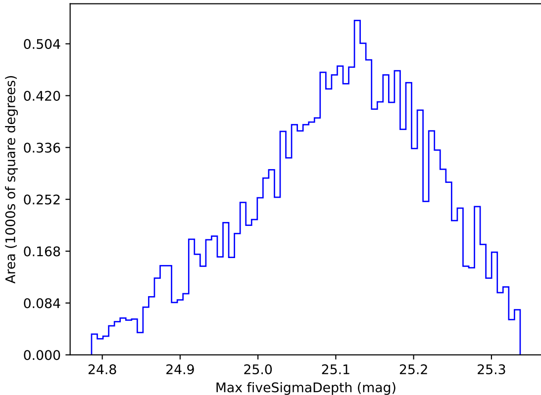
roll_pause_mjdp120_v3.4_10yrs WFD all bands: Max fiveSigmaDepth
