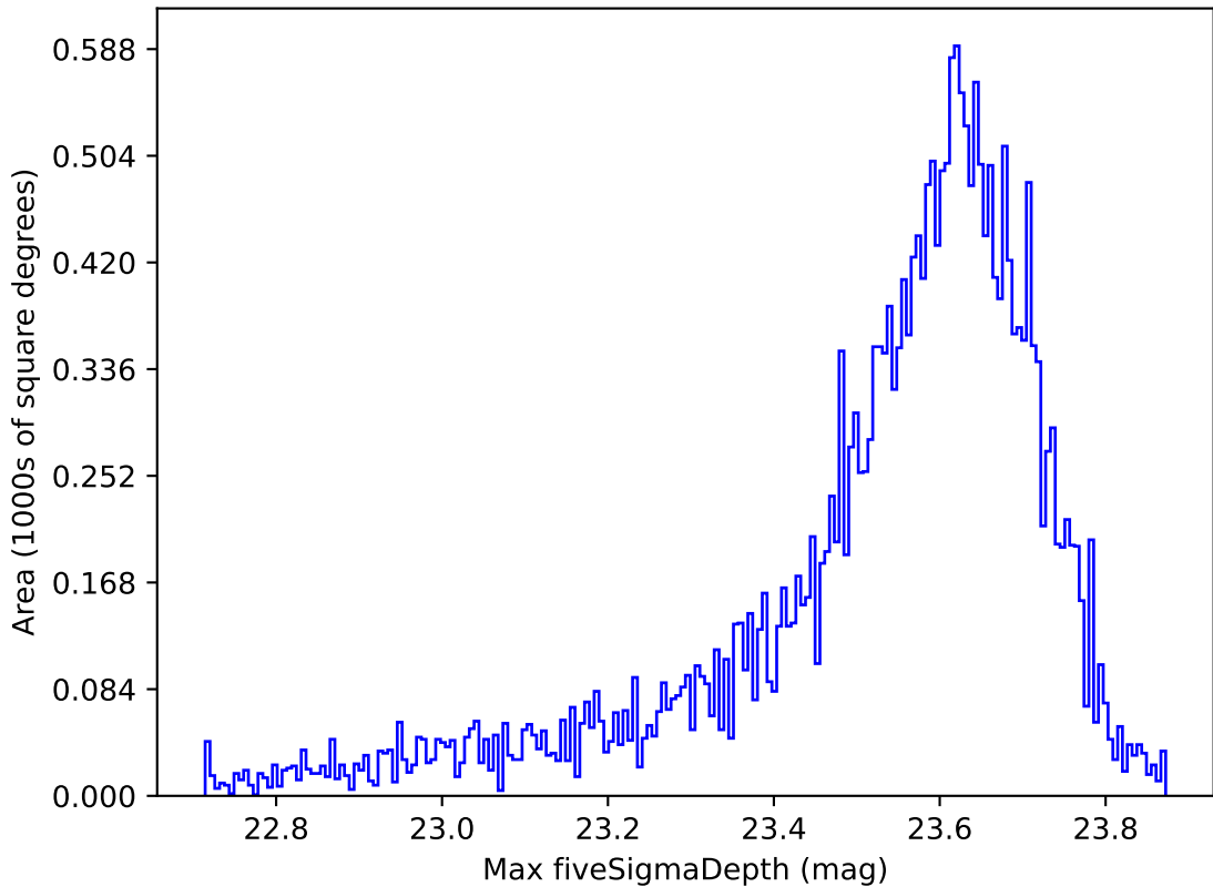
roll_pause_mjdp120_v3.4_10yrs All sky z band: Max fiveSigmaDepth
