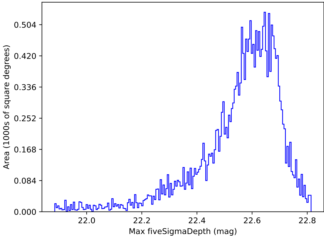
roll_pause_mjdp120_v3.4_10yrs All sky y band: Max fiveSigmaDepth
