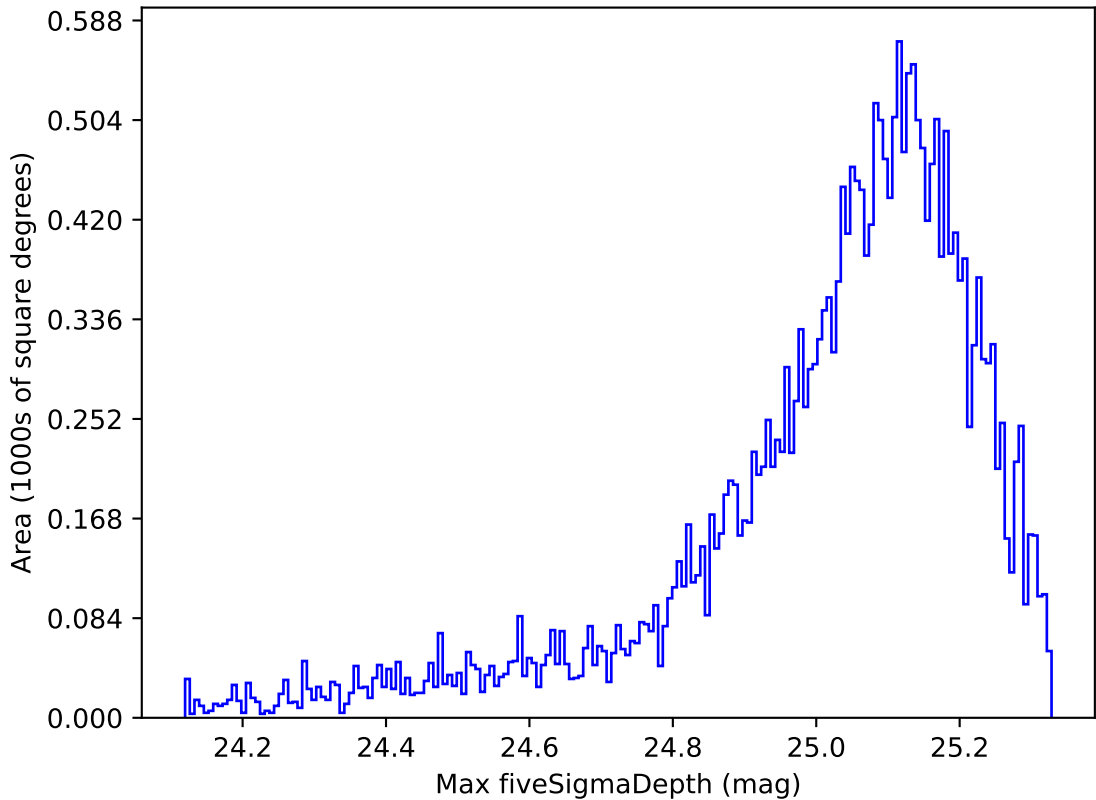
roll_pause_mjdp120_v3.4_10yrs All sky g band: Max fiveSigmaDepth
