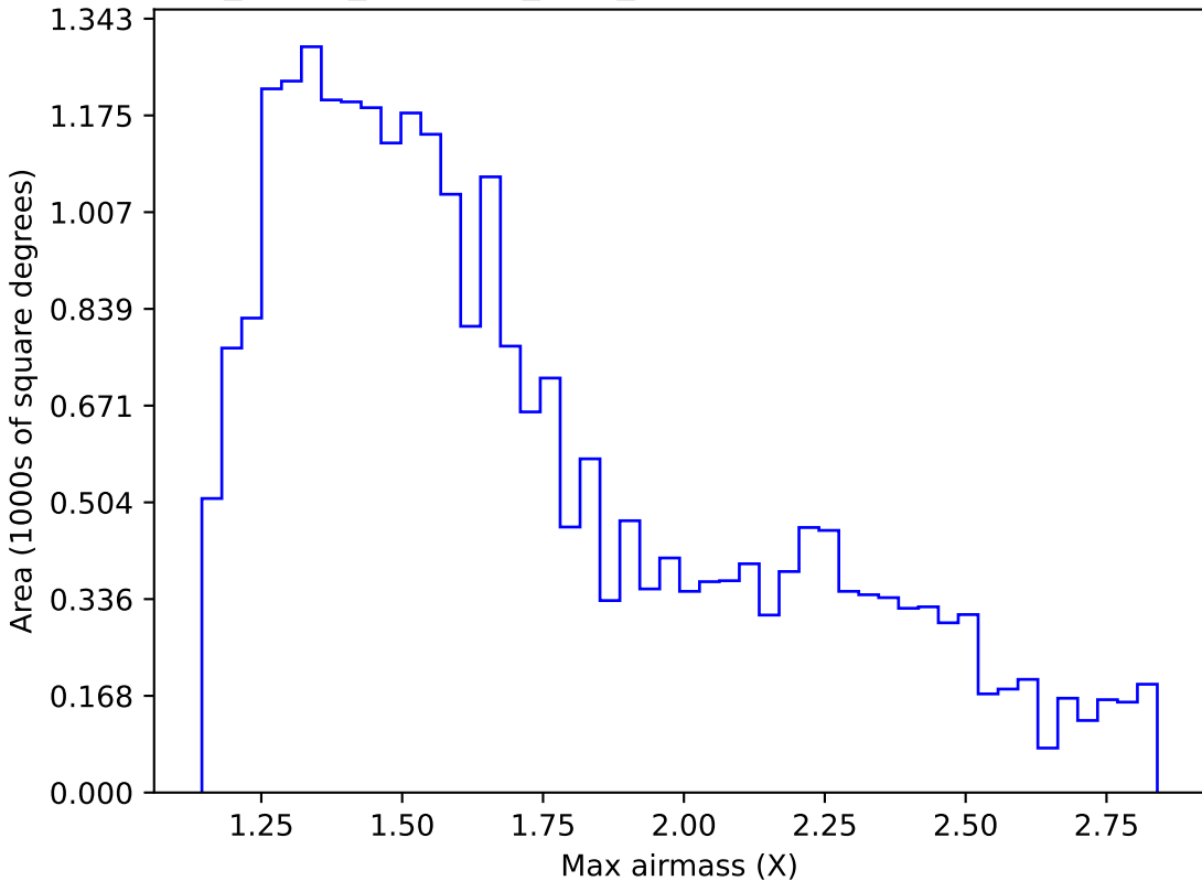
roll_pause_mjdp120_v3.4_10yrs Yr 1 z band: Max airmass
