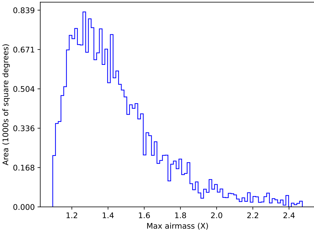
roll_pause_mjdp120_v3.4_10yrs Yr 1 u band: Max airmass
