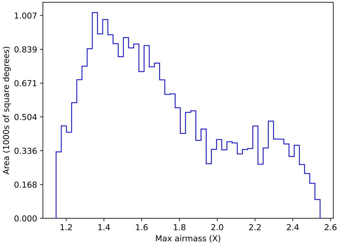
roll_pause_mjdp120_v3.4_10yrs Yr 1 r band: Max airmass
