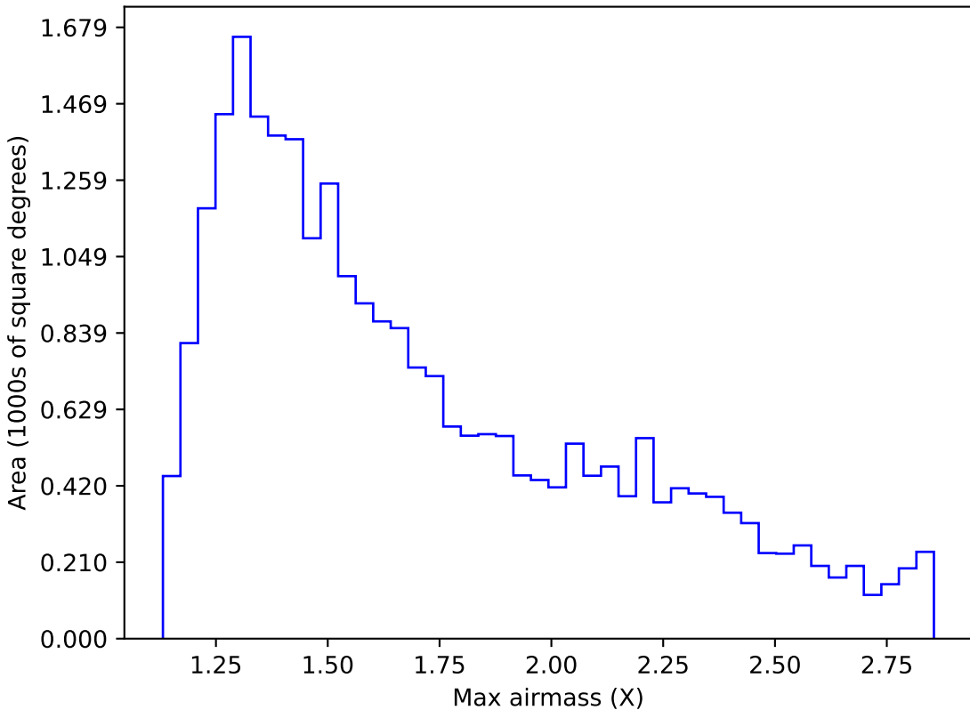
roll_pause_mjdp120_v3.4_10yrs Yr 1 i band: Max airmass
