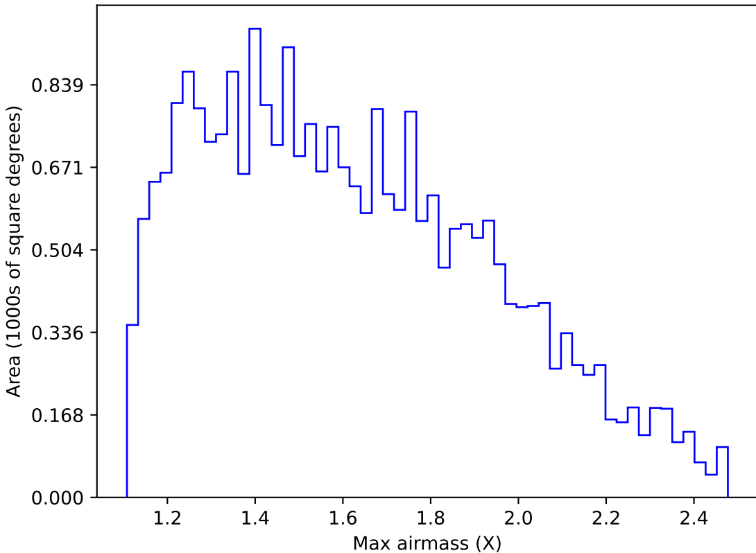
roll_pause_mjdp120_v3.4_10yrs Yr 1 g band: Max airmass
