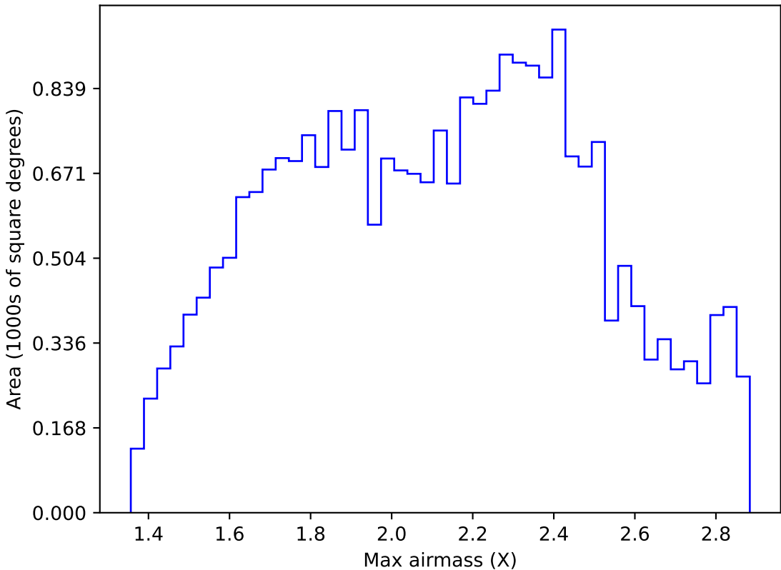
roll_pause_mjdp120_v3.4_10yrs Yr 1 all bands: Max airmass
