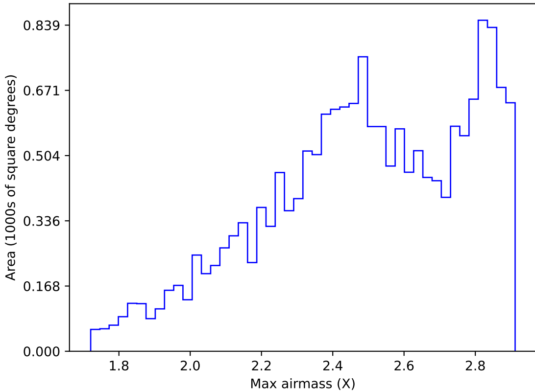
roll_pause_mjdp120_v3.4_10yrs WFD z band: Max airmass
