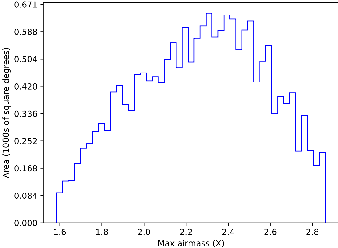
roll_pause_mjdp120_v3.4_10yrs WFD y band: Max airmass
