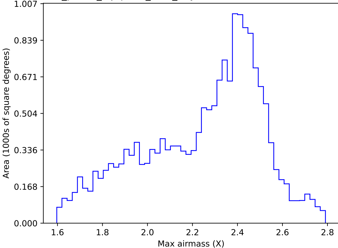
roll_pause_mjdp120_v3.4_10yrs WFD r band: Max airmass
