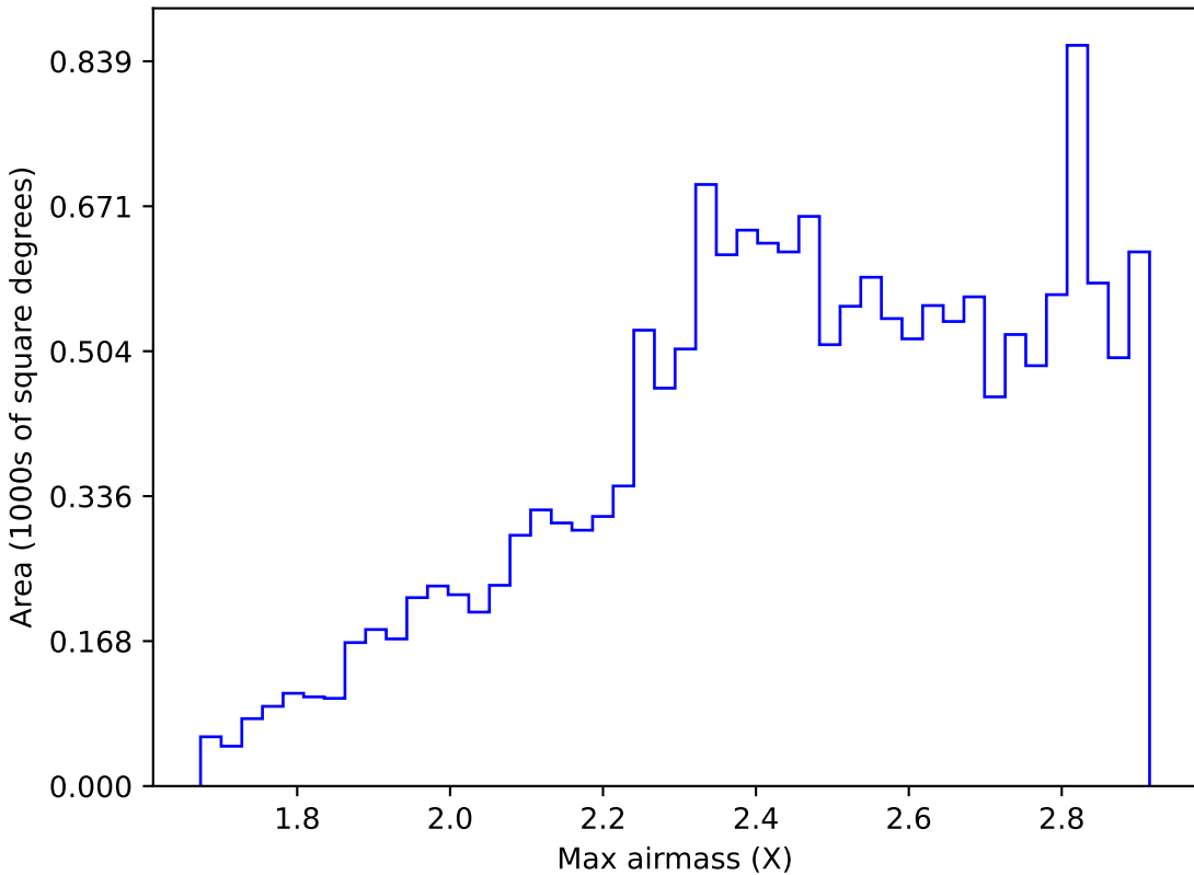
roll_pause_mjdp120_v3.4_10yrs WFD i band: Max airmass
