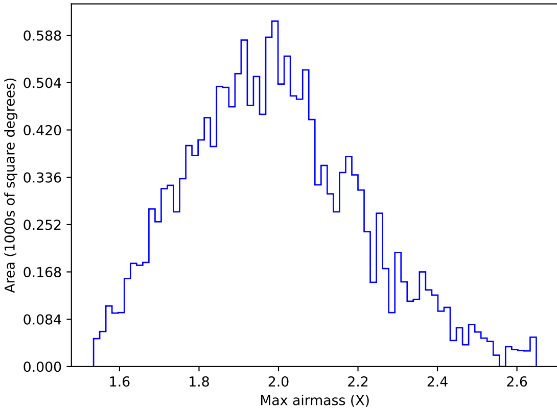
roll_pause_mjdp120_v3.4_10yrs WFD g band: Max airmass
