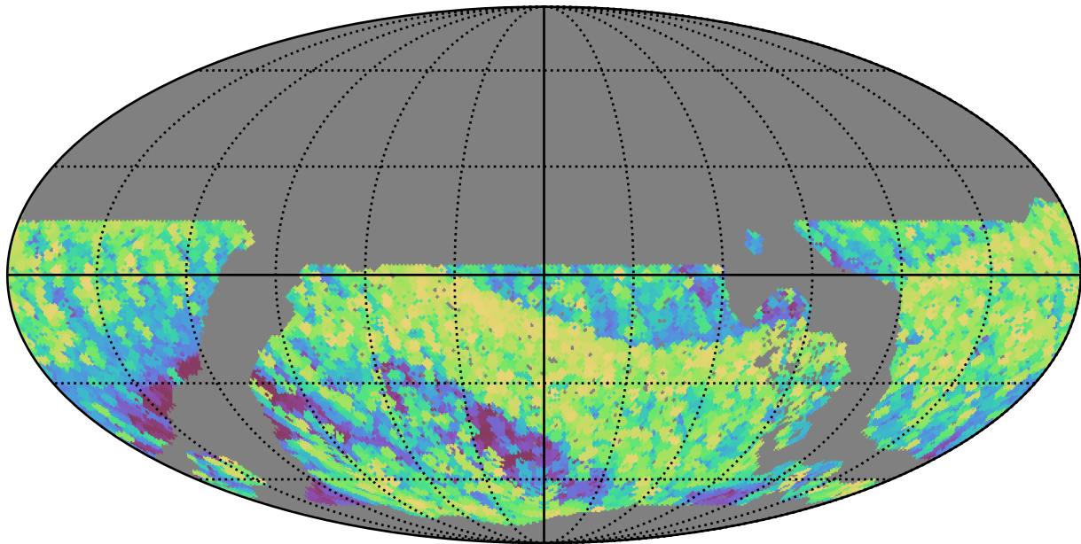
roll_pause_mjdp120_v3.4_10yrs WFD all bands: Max airmass
